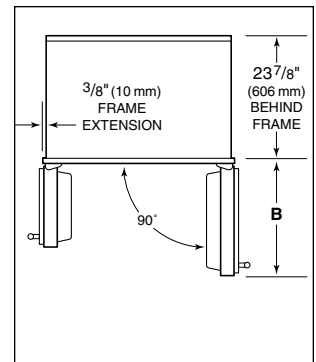
Minimum Door Clearance at 90° – Models 561, 642, 680, 632 and 690
